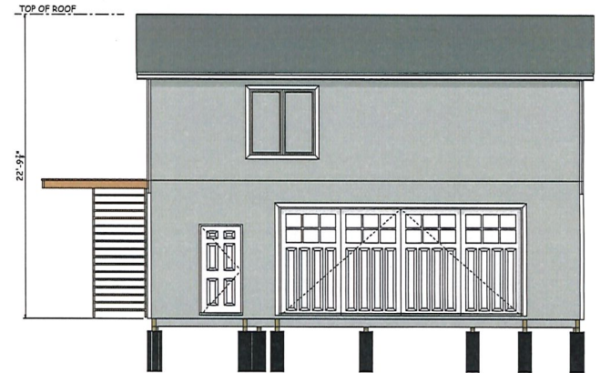
Front Elevation
